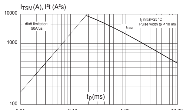
Figure 6. Non-repetitive surge peak on-state current for a sinusoidal pulse
