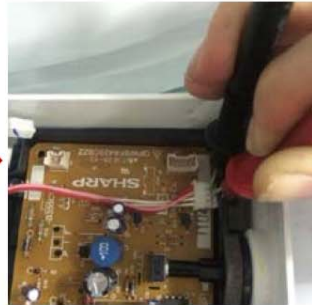
check resistance from pin 3 and 4 at CN3
