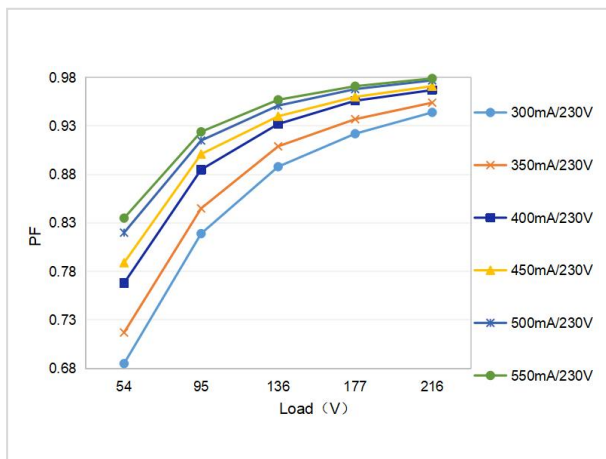
PF Curve 1
