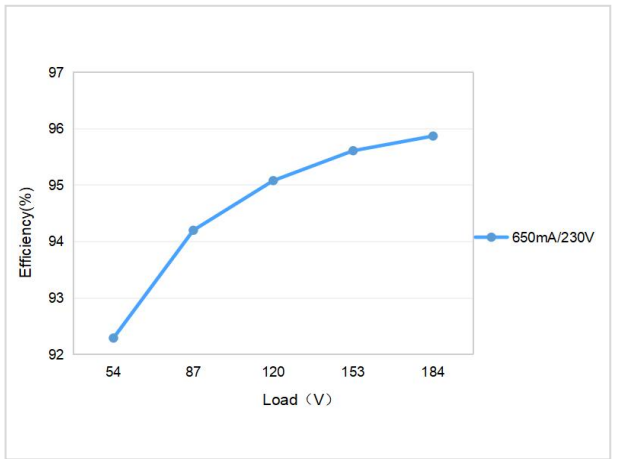
Efficiency Curve 4
