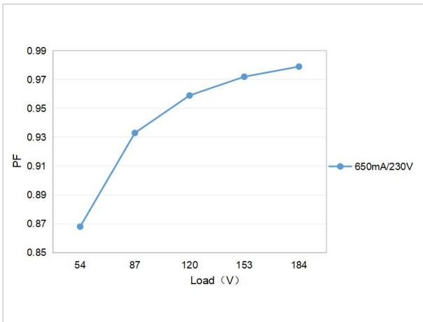
PF Curve 4
