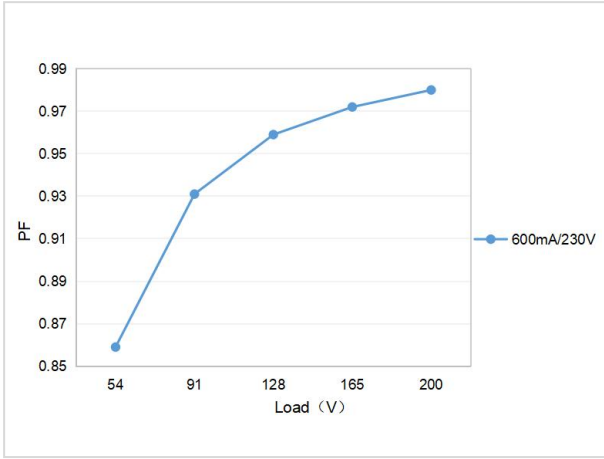
PF Curve 3
