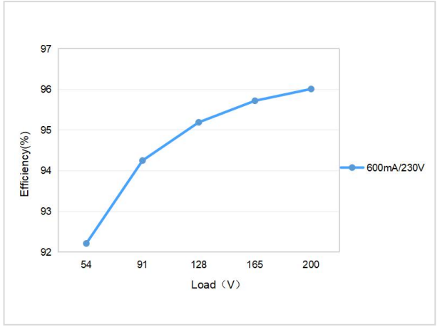
Efficiency Curve 3
